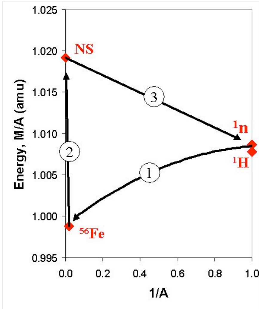
Fig. 4. The nuclear cycle that powers the cosmos: 1. Fusion of lightweight nuclei, like {}^1\text{H} , into heavier ones, like {}^{56}\text{Fe} ; 2. Gravitational collapse of ordinary atomic matter into compact cosmological objects with Z/A = 0 ; and 3. Neutron-emission (and neutron-decay) to produce the hydrogen fuel used in step 1. Charge density, Z/A , declines in steps 1. and 2. from Z/A = 1 to Z/A = 0 , but Z/A is unchanged in step 3., neutron-emission. Fragmentation [10-15] of super-massive neutron stars into smaller ones is not shown.
