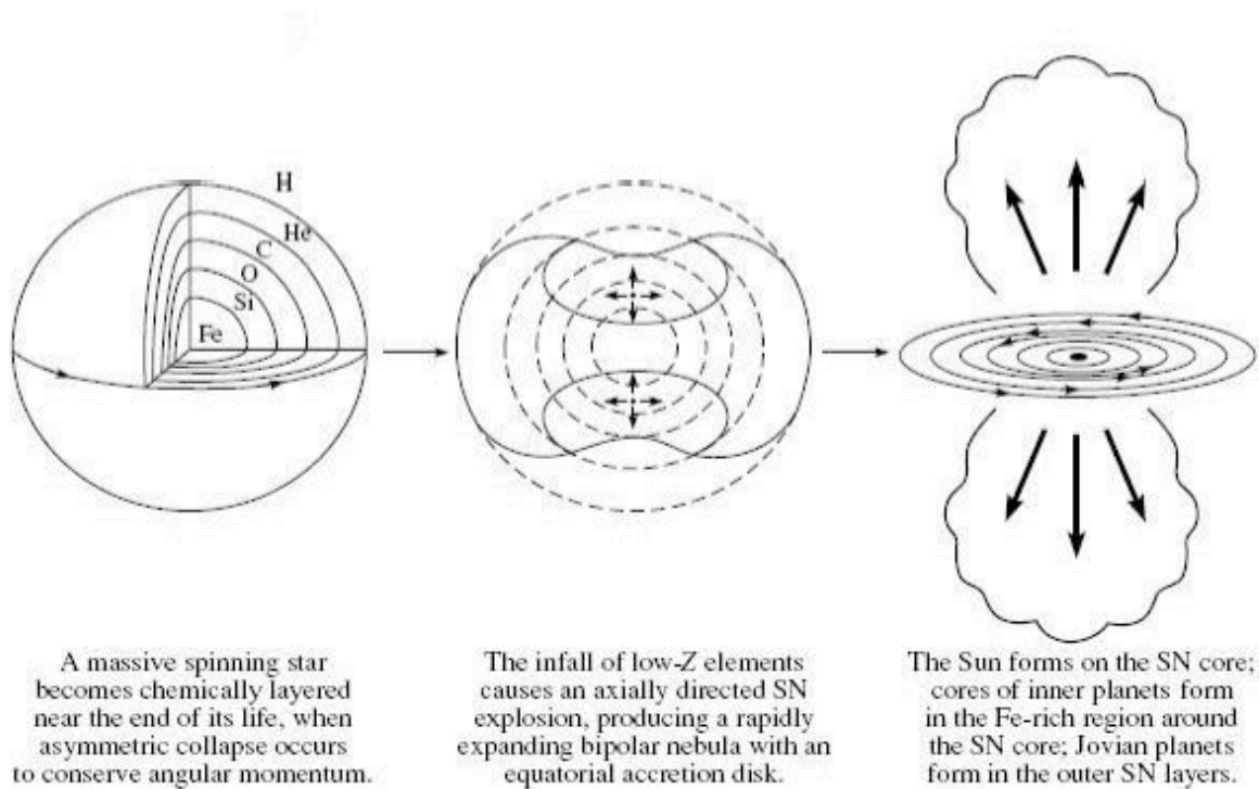
Fig. 1. A scenario proposed in the mid-1970s to explain the unexpected link observed between specific isotopes of heavy elements with light element abundances in meteorites at the birth of the solar system [20-21]. According to this view, the Sun is iron-rich and formed on the collapsed core of a supernova (SN), material near the SN core formed iron cores of the planets near the Sun, and light elements from the outer SN layers formed the giant Jovian planets.
